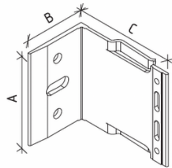
Double fixing bracket
