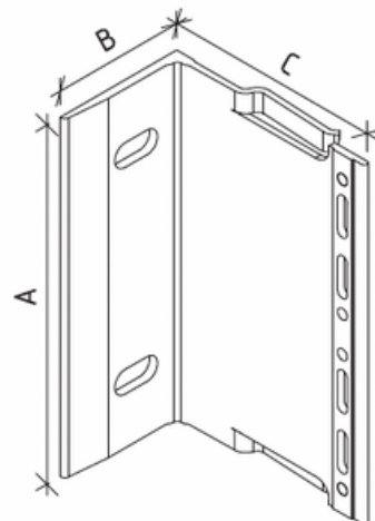
Double fixing bracket
